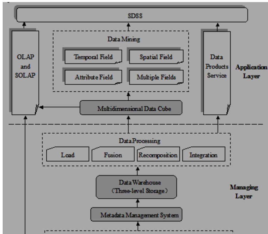
Figure 1: A Spatial Data Warehouse Architecture
